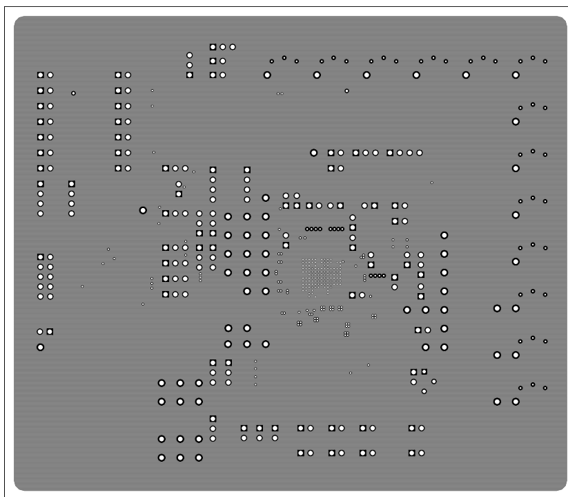
Figure 14. Layer 2
