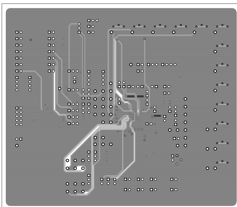
Figure 17. Layer 5
