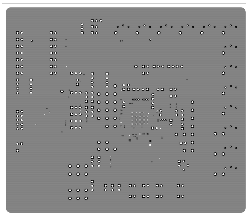
Figure 15. Layer 3
