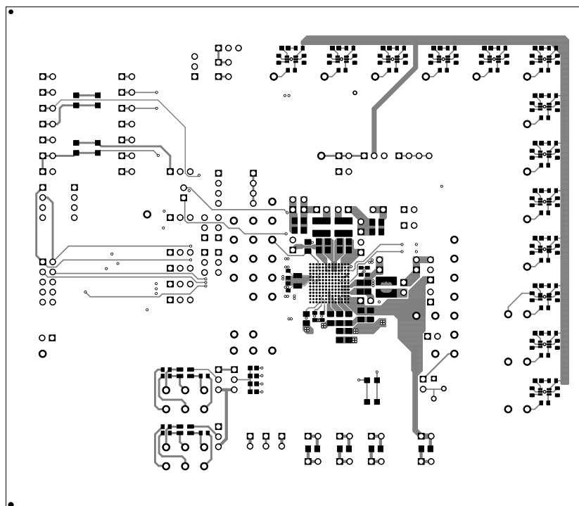
Figure 13. Top Layer
