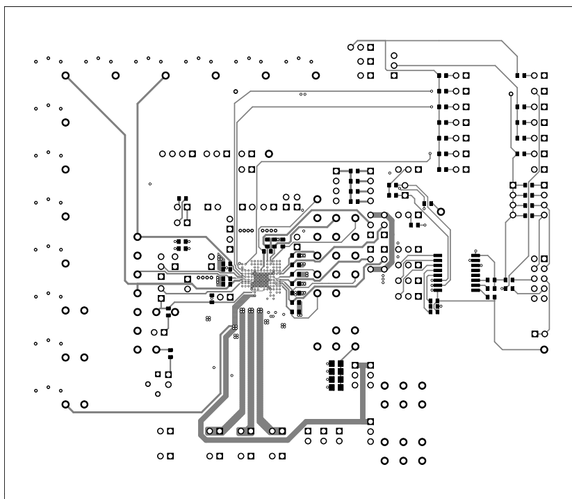
Figure 18. Layer 6
